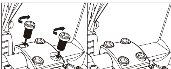
Head Tube Installation Illustration
